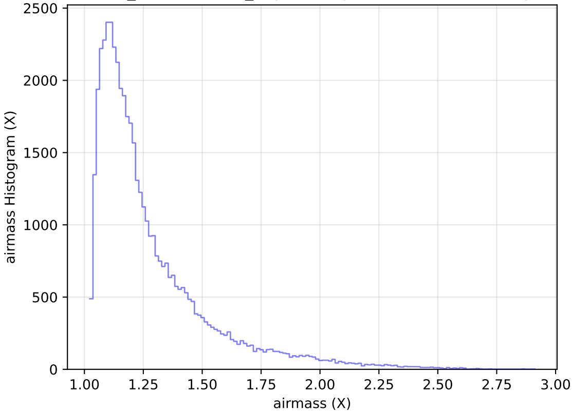
weather_cloudso6v3.4_10yrs Yr 1 y band: airmass Histogram
