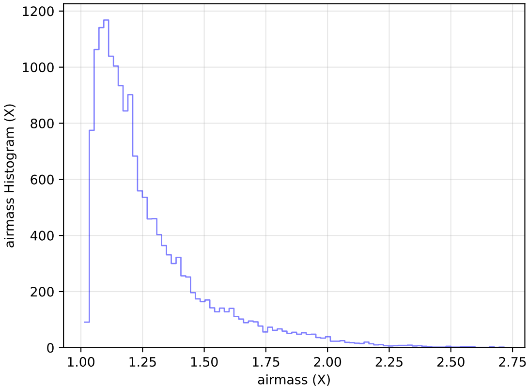
weather_cloudso6v3.4_10yrs Yr 1 u band: airmass Histogram
