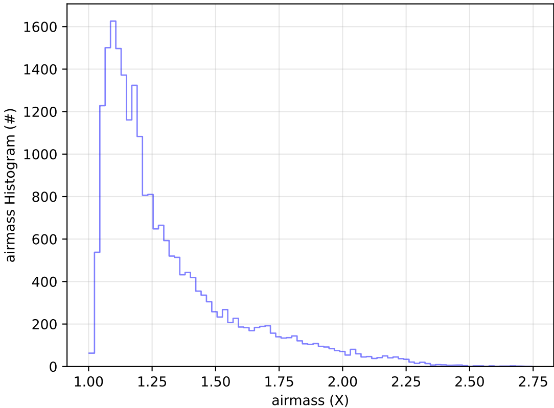
weather_cloudso6v3.4_10yrs Yr 1 g band: airmass Histogram
