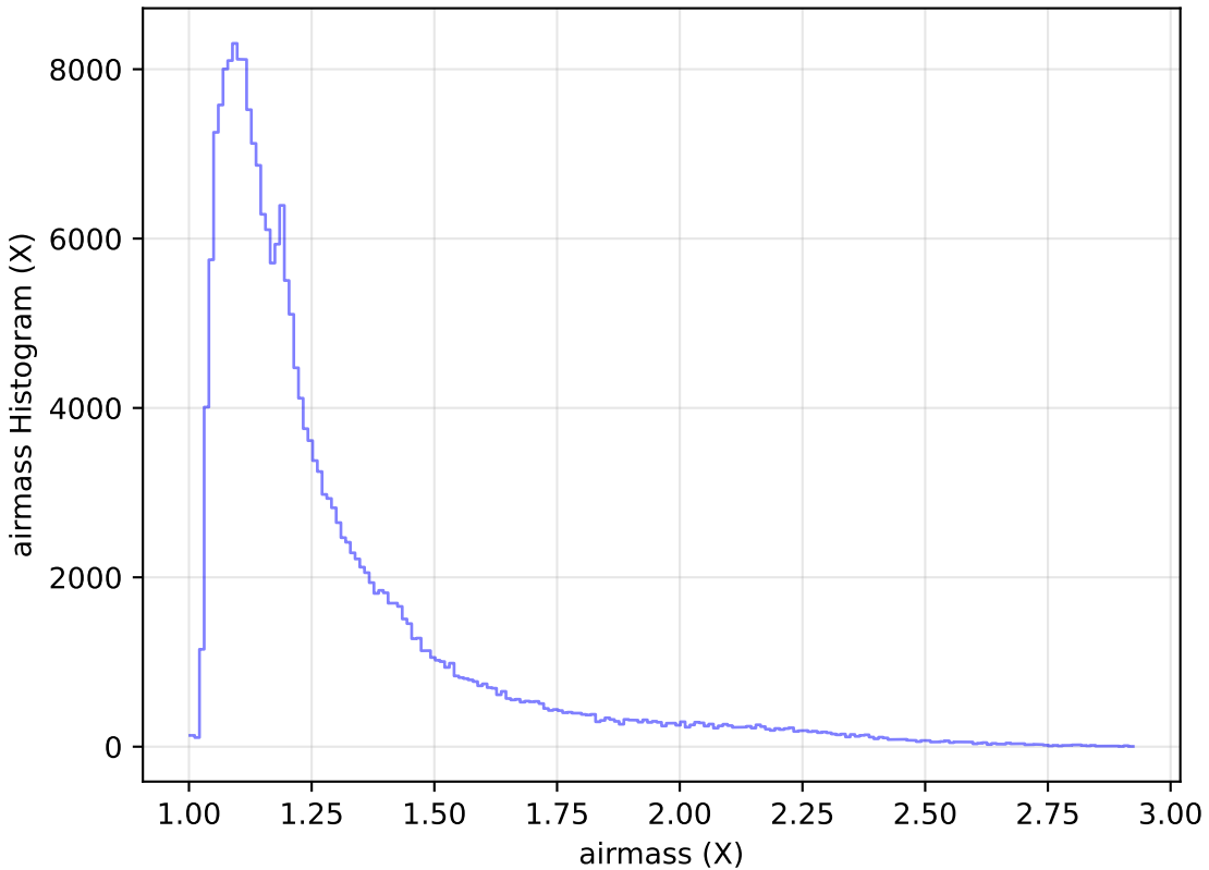
weather_cloudso6v3.4_10yrs Yr 1 all bands: airmass Histogram
