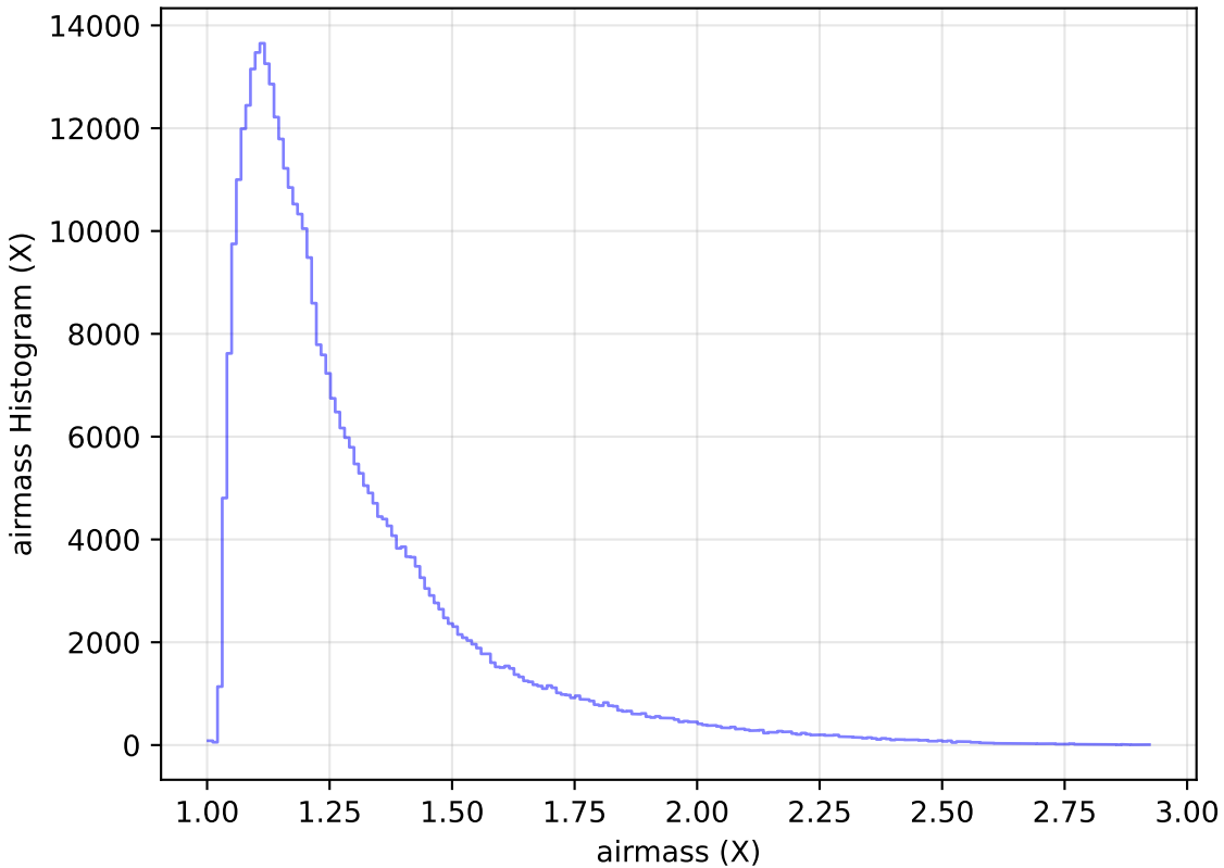
weather_cloudso6v3.4_10yrs WFD y band: airmass Histogram
