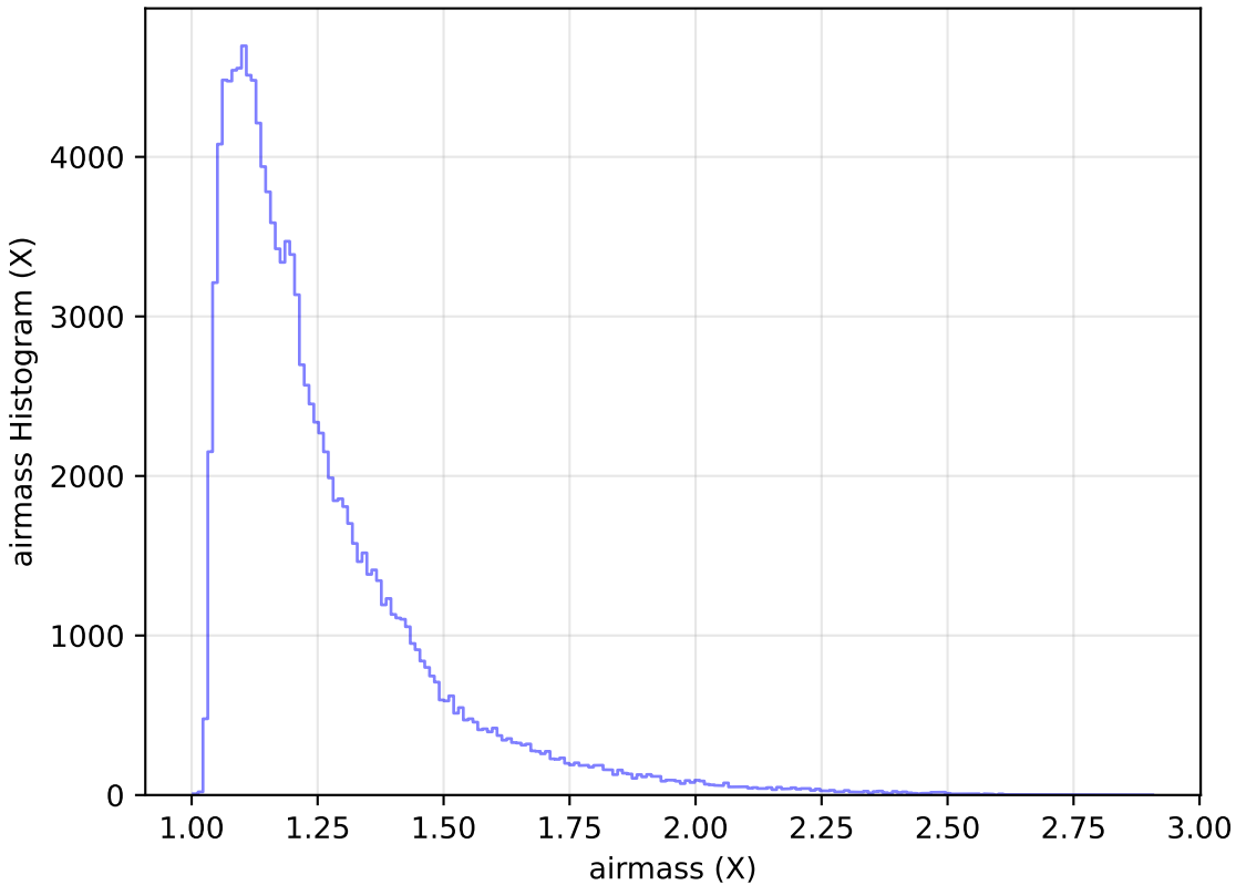
weather_cloudso6v3.4_10yrs WFD u band: airmass Histogram
