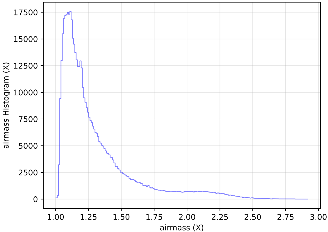
weather_cloudso6v3.4_10yrs WFD r band: airmass Histogram
