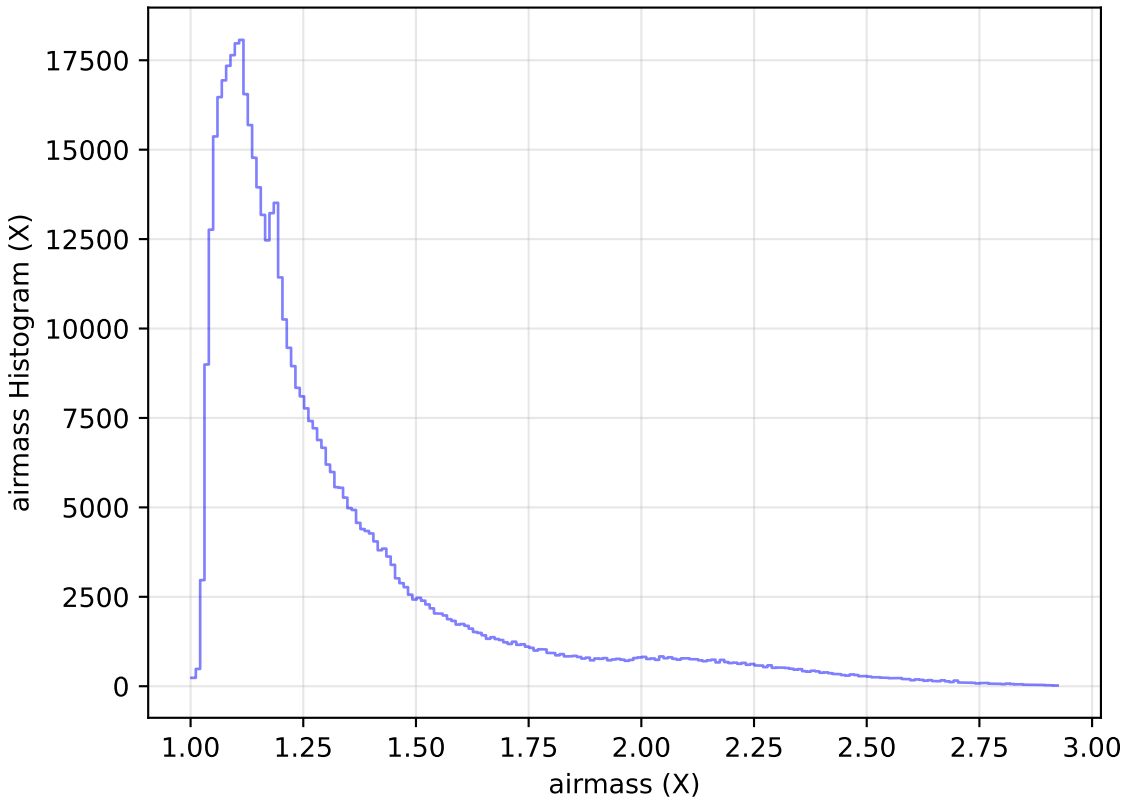
weather_cloudso6v3.4_10yrs WFD i band: airmass Histogram
