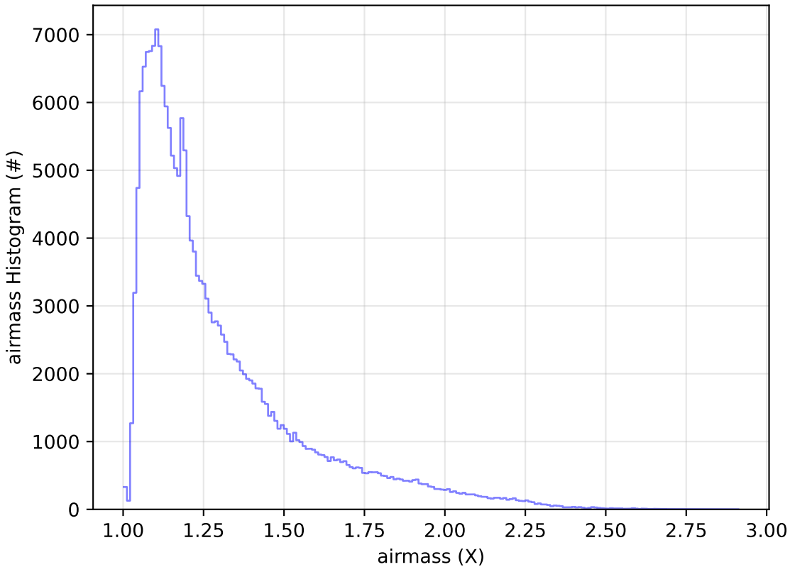
weather_cloudso6v3.4_10yrs WFD g band: airmass Histogram
