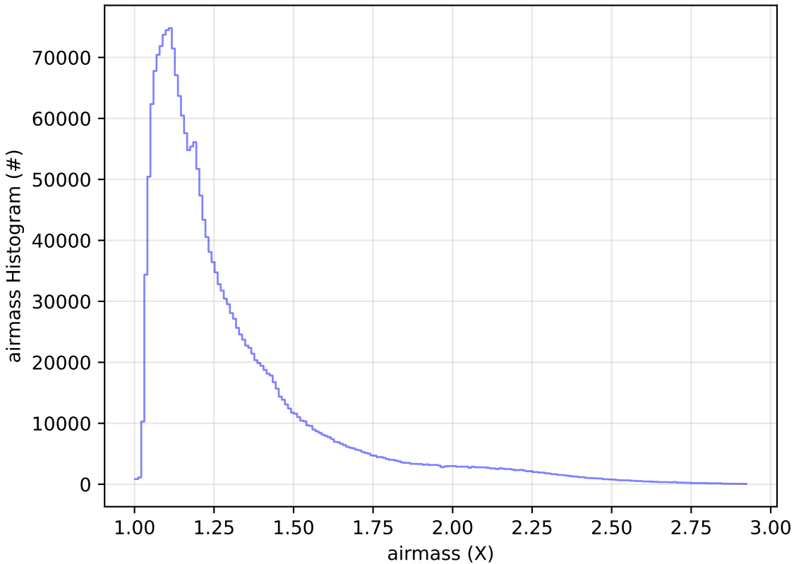
weather_cloudso6v3.4_10yrs WFD all bands: airmass Histogram
