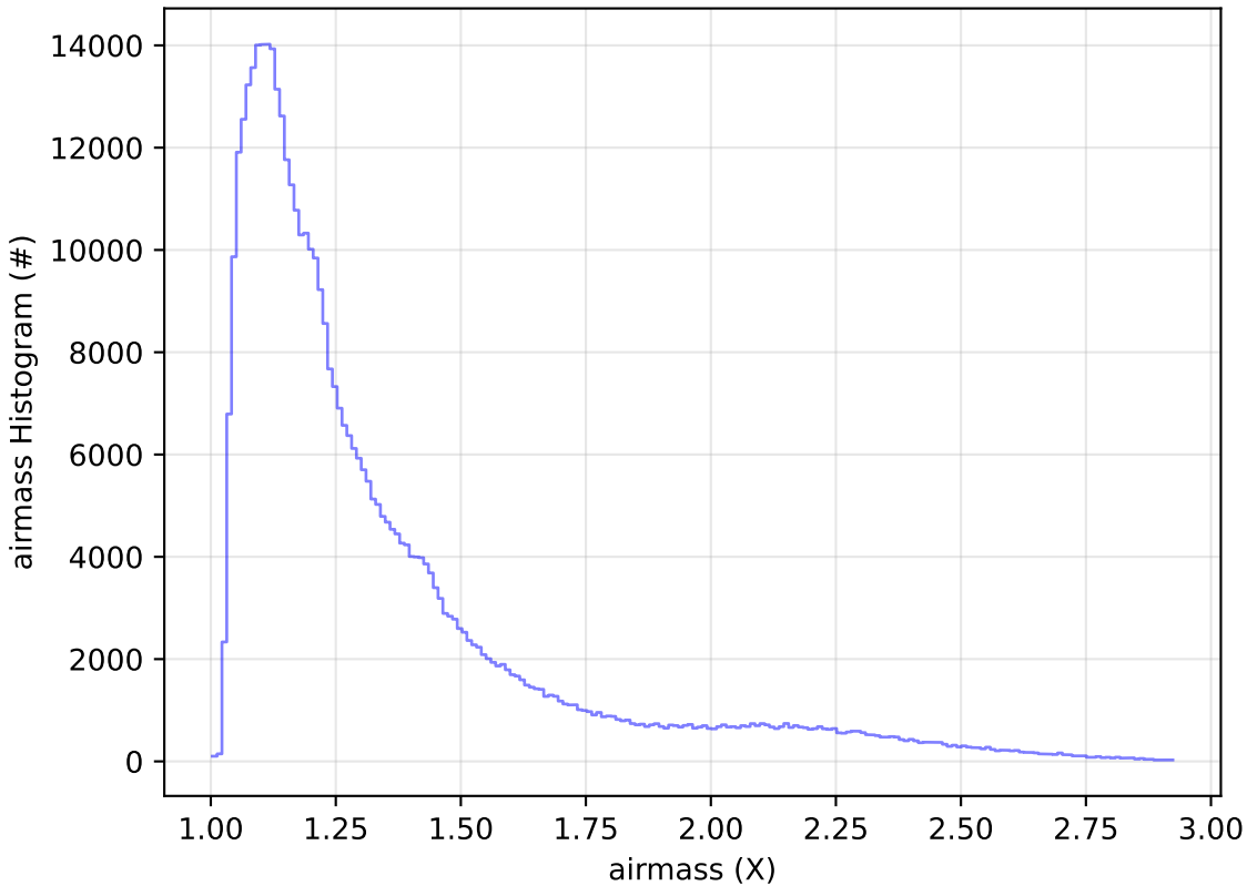
weather_cloudso6v3.4_10yrs All sky z band: airmass Histogram
