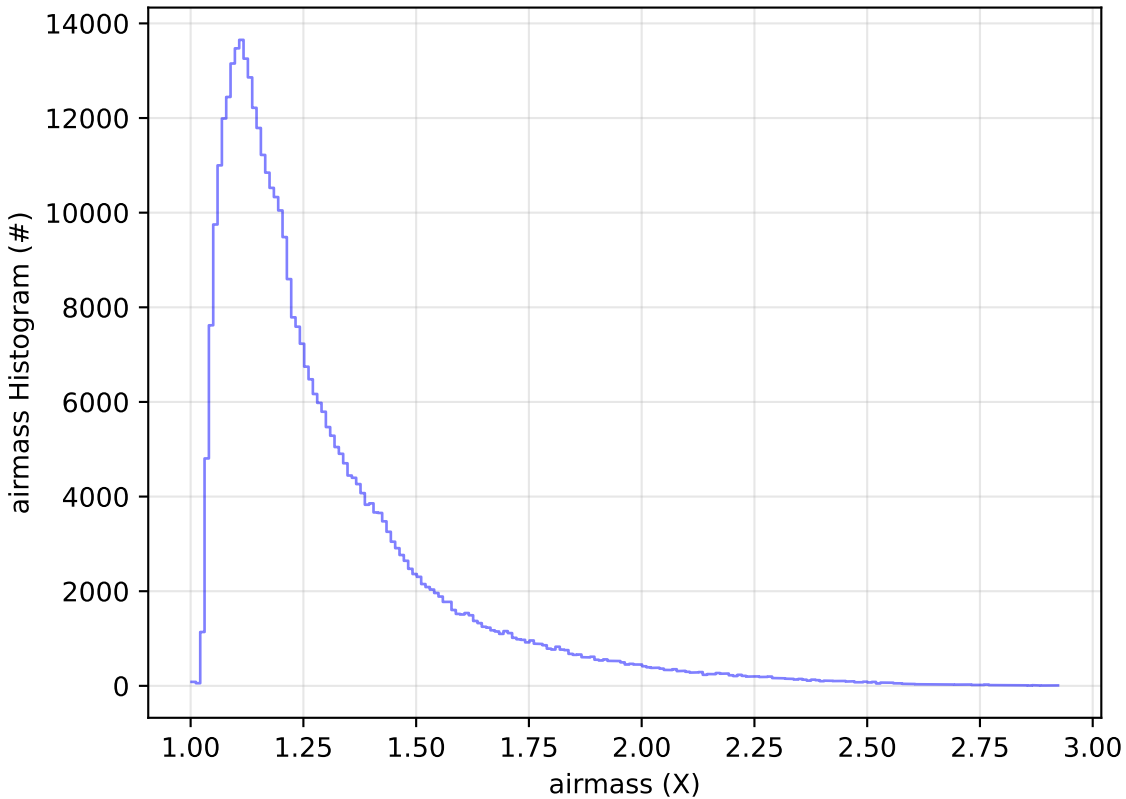
weather_cloudso6v3.4_10yrs All sky y band: airmass Histogram
