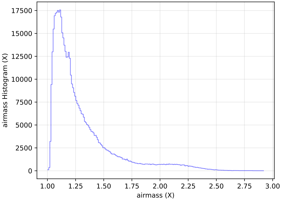
weather_cloudso6v3.4_10yrs All sky r band: airmass Histogram
