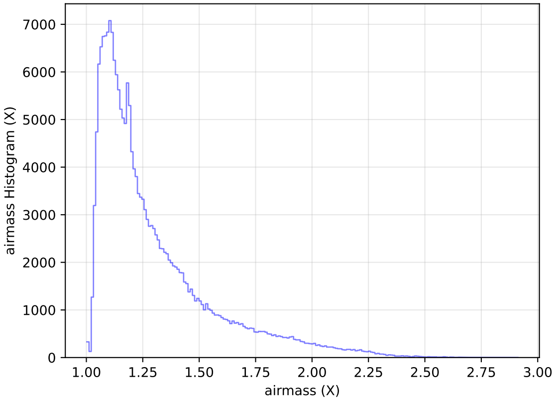
weather_cloudso6v3.4_10yrs All sky g band: airmass Histogram
