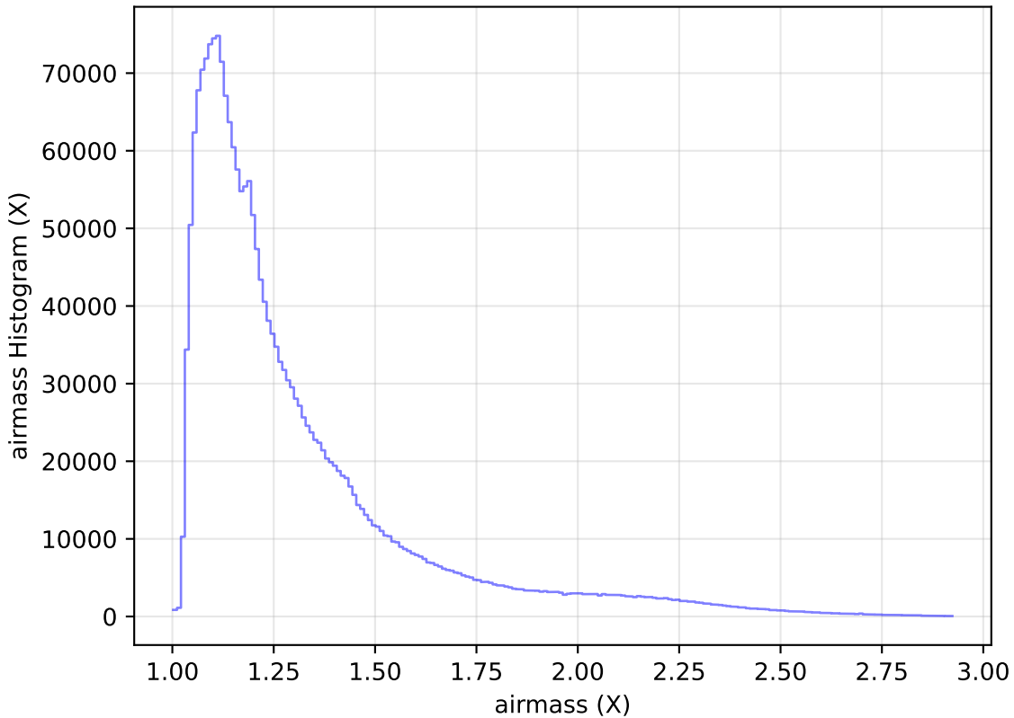
weather_cloudso6v3.4_10yrs All sky all bands: airmass Histogram
