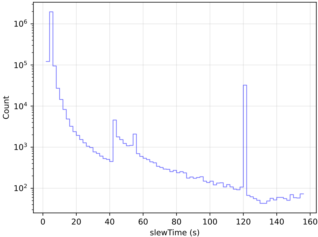
weather_cloudso6v3.4_10yrs All visits: Slew Time Histogram
