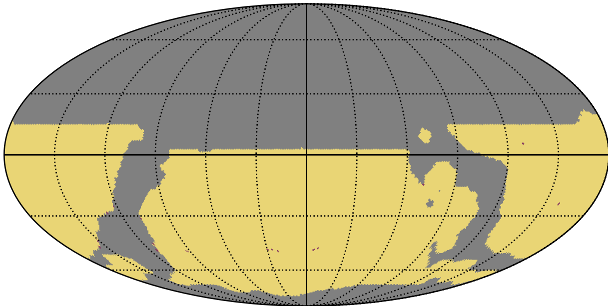
weather_cloudso6v3.4_10yrs WFD: RapidRevisits
