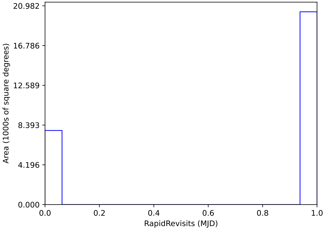
weather_cloudso6v3.4_10yrs All sky: RapidRevisits
