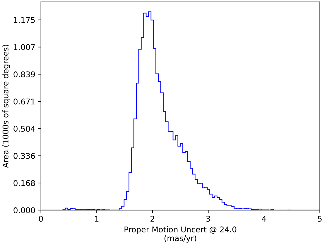
weather_cloudso6v3.4_10yrs WFD: Proper Motion Uncert @ 24.0
