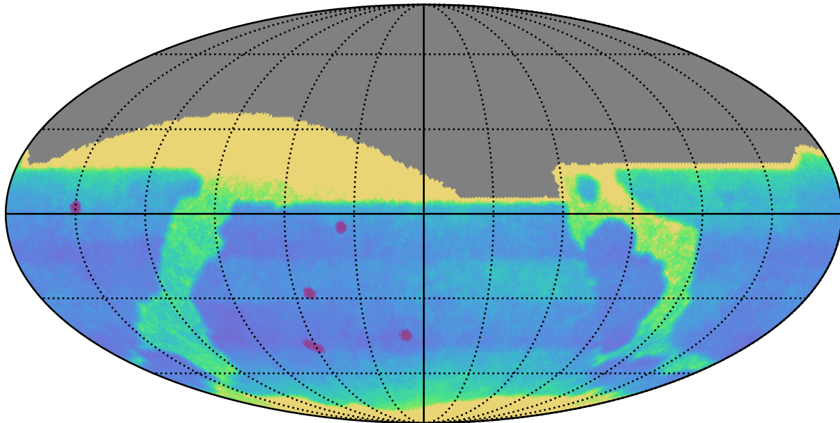
weather_cloudso6v3.4_10yrs All sky: Proper Motion Uncert @ 24.0
