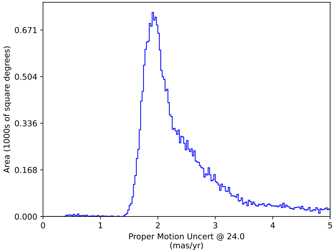
weather_cloudso6v3.4_10yrs All sky: Proper Motion Uncert @ 24.0
