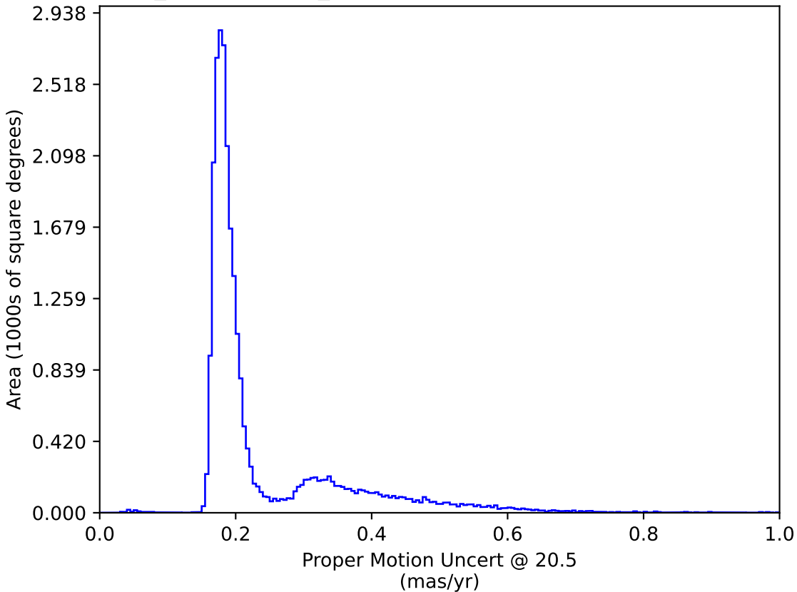
weather_cloudso6v3.4_10yrs All sky: Proper Motion Uncert @ 20.5
