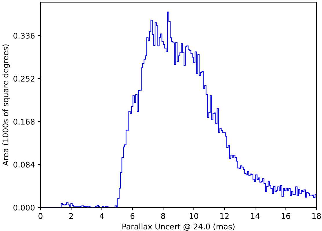
weather_cloudso6v3.4_10yrs All sky: Parallax Uncert @ 24.0
