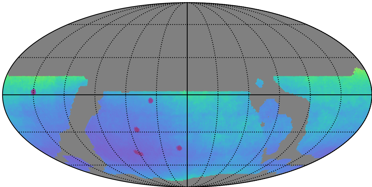
weather_cloudso6v3.4_10yrs WFD: Parallax Uncert @ 22.4
