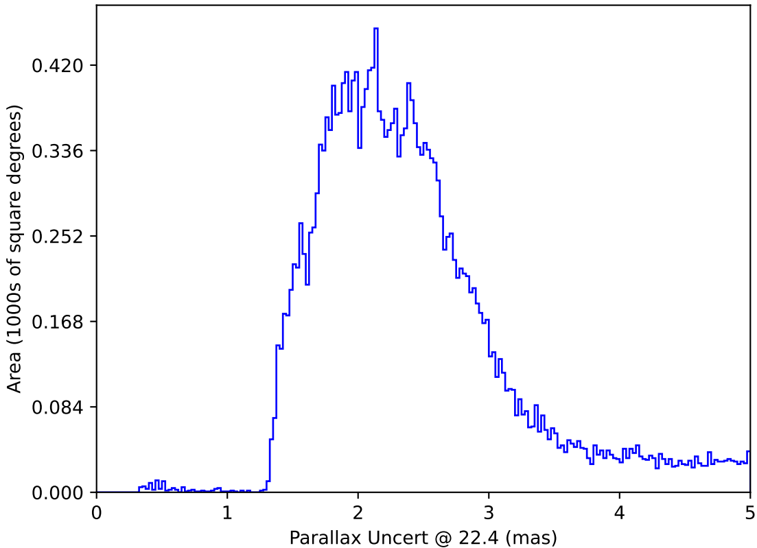
weather_cloudso6v3.4_10yrs All sky: Parallax Uncert @ 22.4
