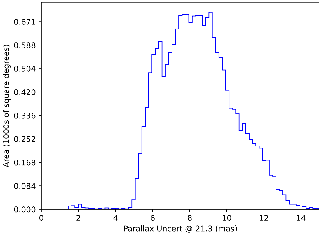
weather_cloudso6v3.4_10yrs WFD y band only: Parallax Uncert @ 21.3
