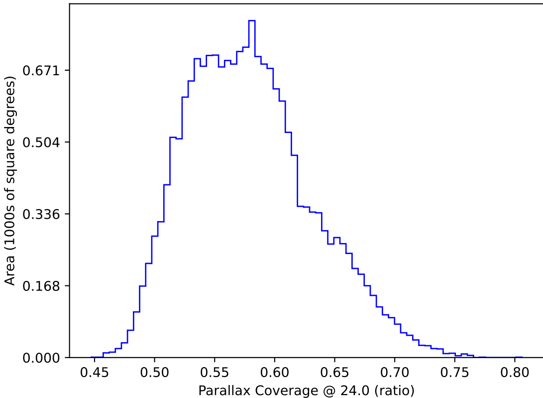
weather_cloudso6v3.4_10yrs WFD: Parallax Coverage @ 24.0
