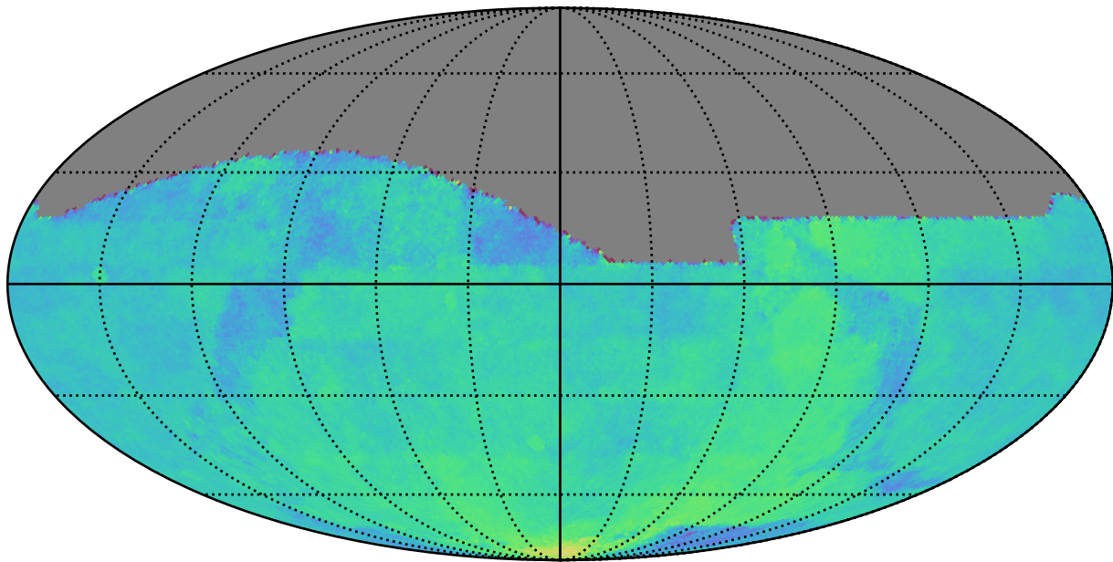
weather_cloudso6v3.4_10yrs All sky: Parallax Coverage @ 24.0
