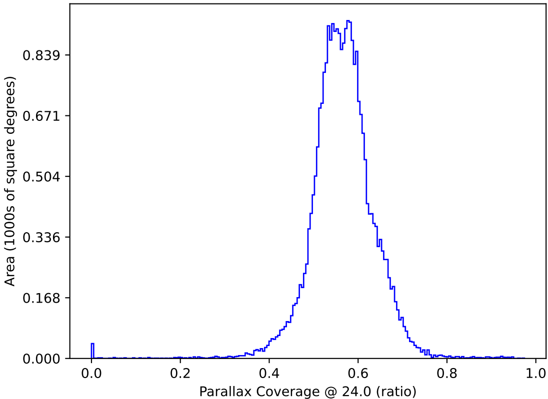
weather_cloudso6v3.4_10yrs All sky: Parallax Coverage @ 24.0
