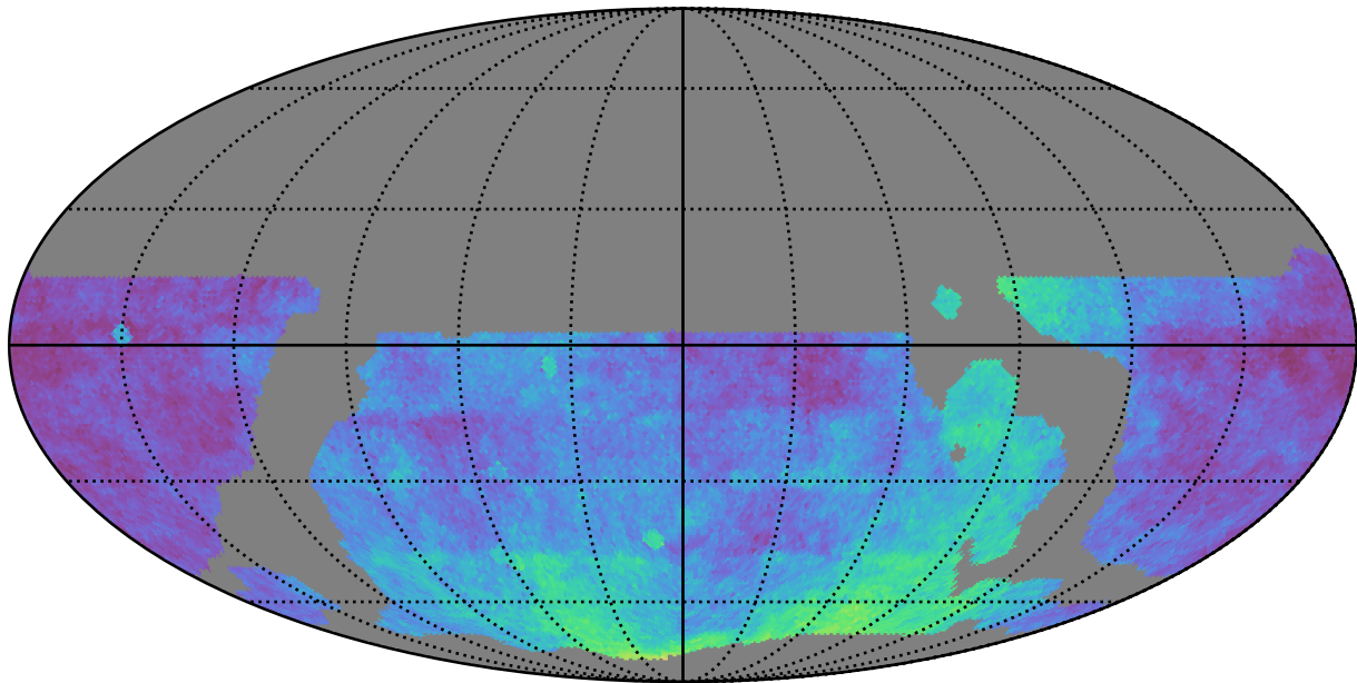
weather_cloudso6v3.4_10yrs WFD: Parallax Coverage @ 22.4
