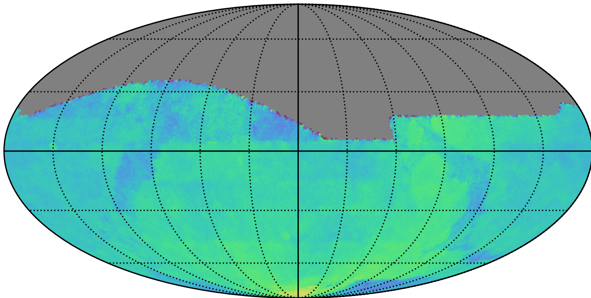
weather_cloudso6v3.4_10yrs All sky: Parallax Coverage @ 22.4
