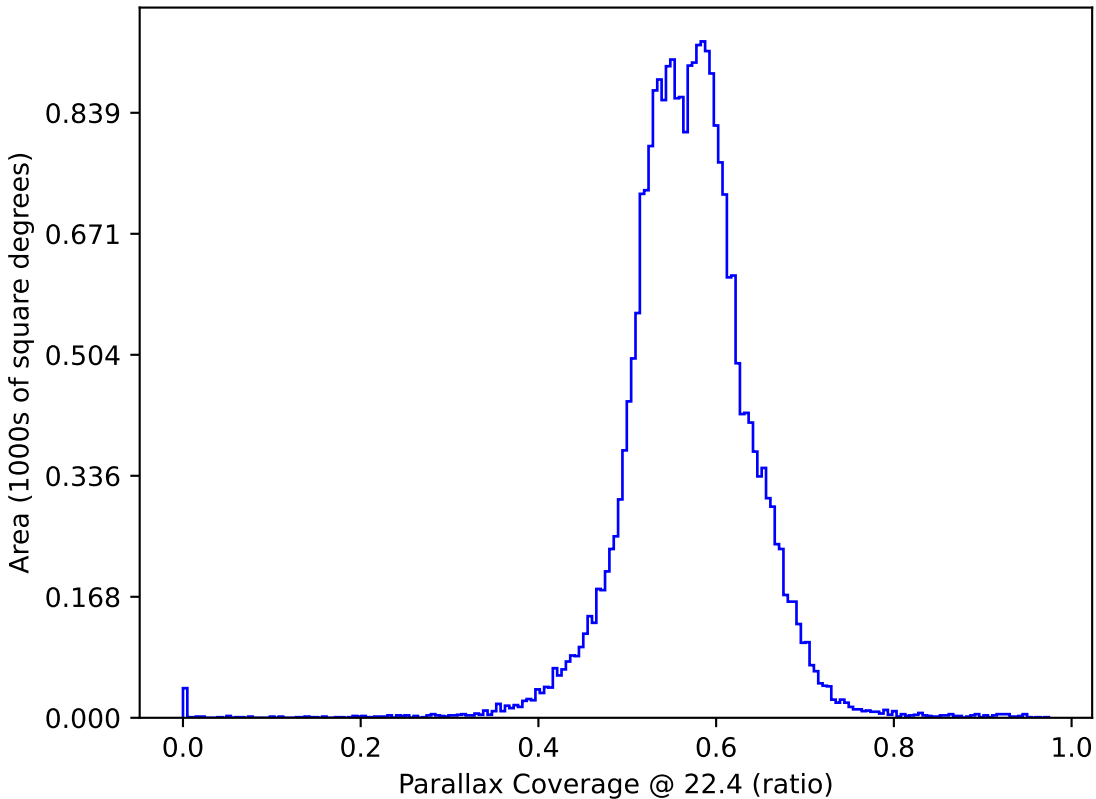
weather_cloudso6v3.4_10yrs All sky: Parallax Coverage @ 22.4
