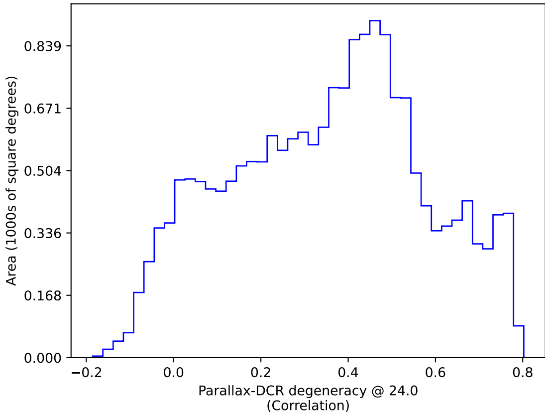
weather_cloudso6v3.4_10yrs WFD: Parallax-DCR degeneracy @ 24.0
