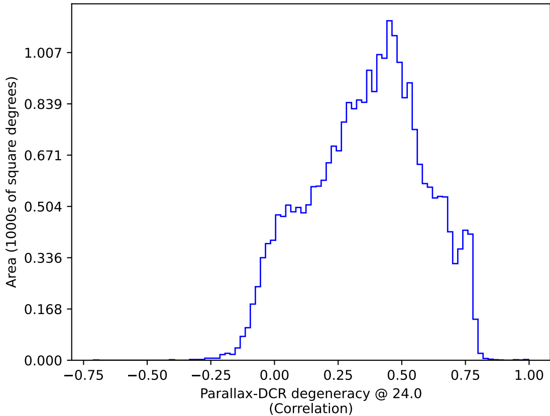
weather_cloudso6v3.4_10yrs All sky: Parallax-DCR degeneracy @ 24.0
