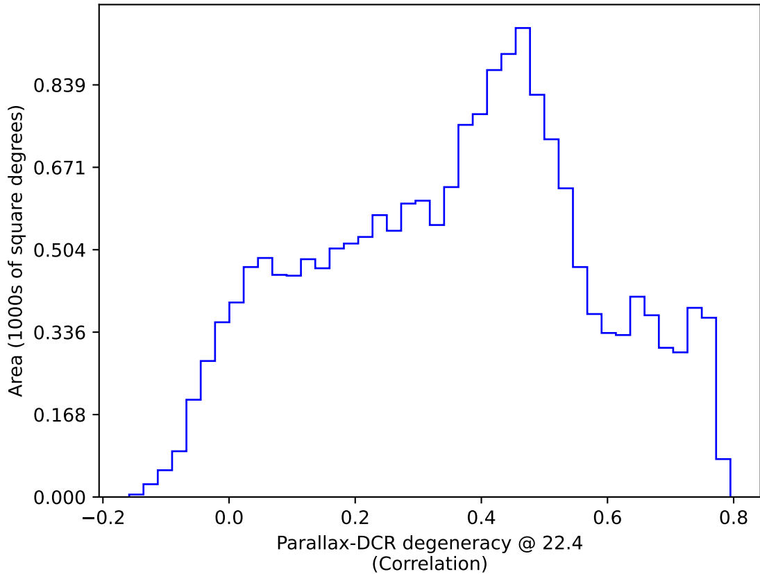
weather_cloudso6v3.4_10yrs WFD: Parallax-DCR degeneracy @ 22.4
