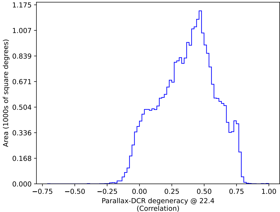
weather_cloudso6v3.4_10yrs All sky: Parallax-DCR degeneracy @ 22.4
