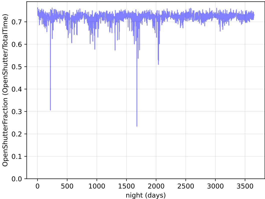
weather_cloudso6v3.4_10yrs Per night: OpenShutterFraction
