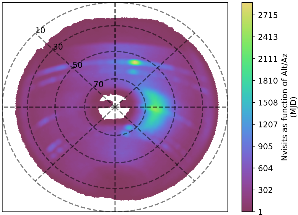
weather_cloudso6v3.4_10yrs z band: Nvisits as function of Alt/Az
