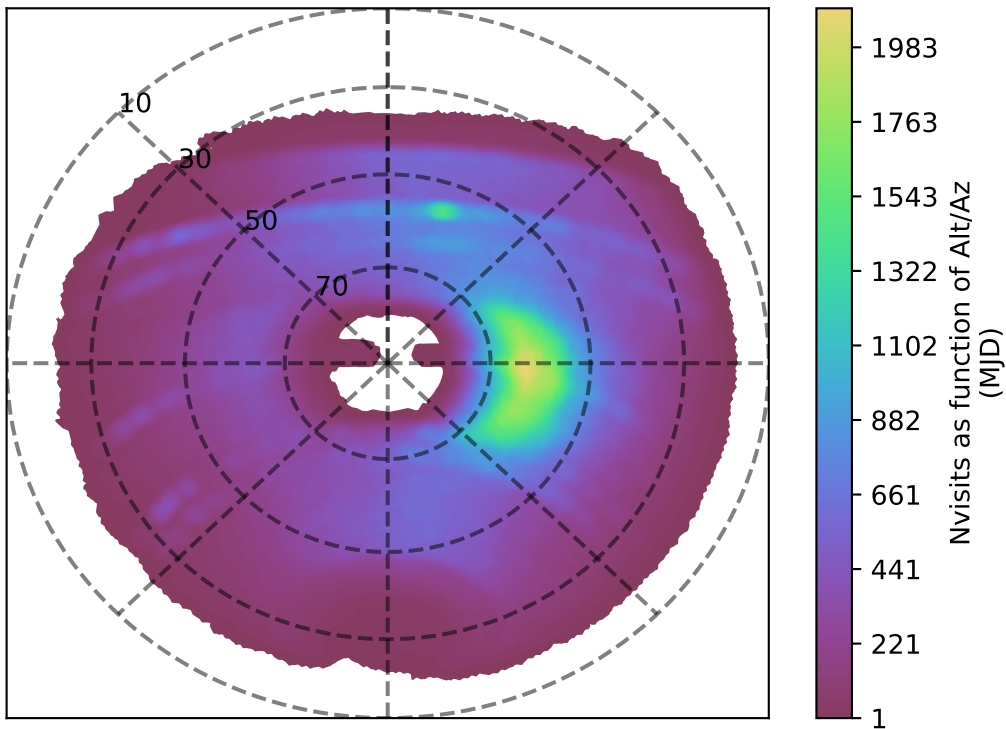
weather_cloudso6v3.4_10yrs y band: Nvisits as function of Alt/Az
