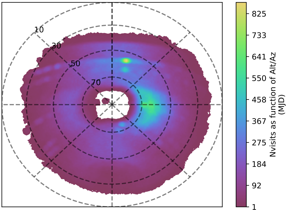
weather_cloudso6v3.4_10yrs u band: Nvisits as function of Alt/Az
