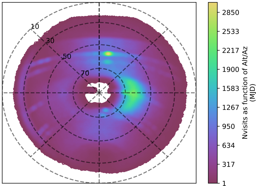
weather_cloudso6v3.4_10yrs r band: Nvisits as function of Alt/Az
