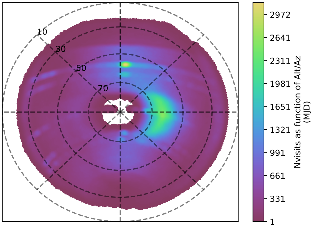
weather_cloudso6v3.4_10yrs i band: Nvisits as function of Alt/Az
