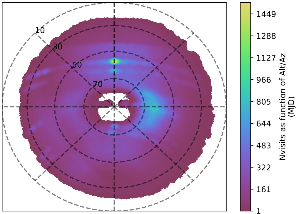
weather_cloudso6v3.4_10yrs g band: Nvisits as function of Alt/Az
