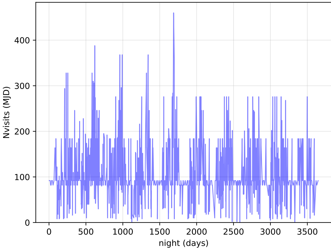
weather_cloudso6v3.4_10yrs DDF: Nvisits
