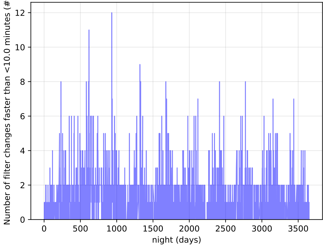
weather_cloudso6v3.4_10yrs Per Night: Number of filter changes faster than <10.0 minutes
