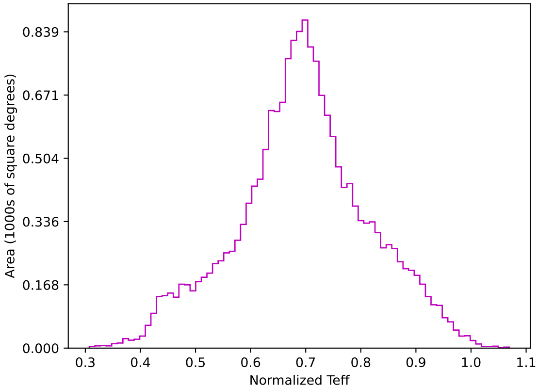
weather_cloudso6v3.4_10yrs WFD z band: Normalized Teff
