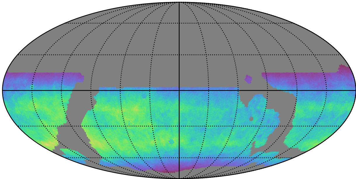
weather_cloudso6v3.4_10yrs WFD y band: Normalized Teff
