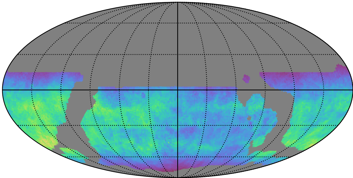
weather_cloudso6v3.4_10yrs WFD u band: Normalized Teff
