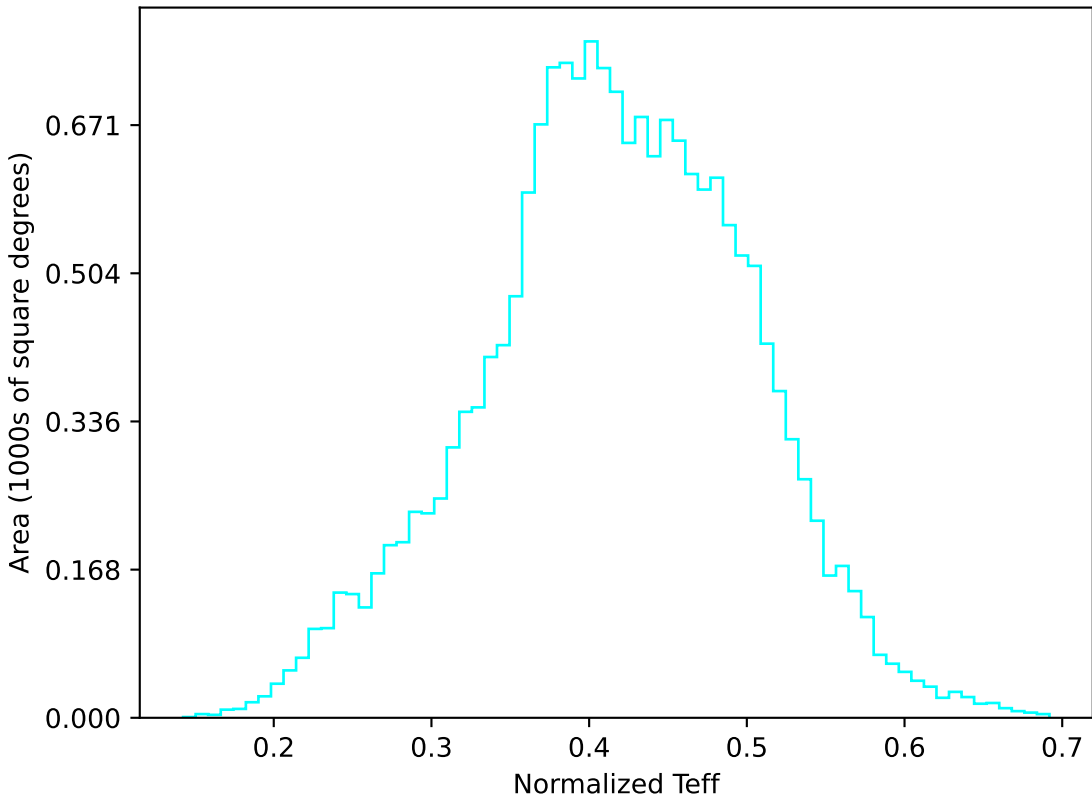
weather_cloudso6v3.4_10yrs WFD u band: Normalized Teff
