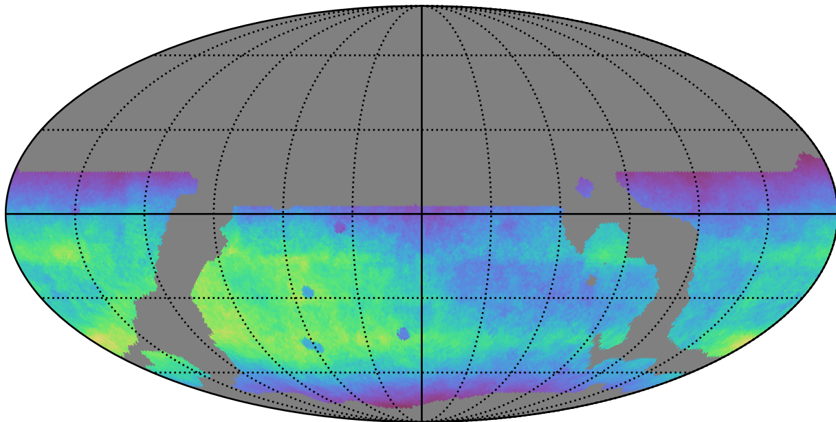
weather_cloudso6v3.4_10yrs WFD r band: Normalized Teff
